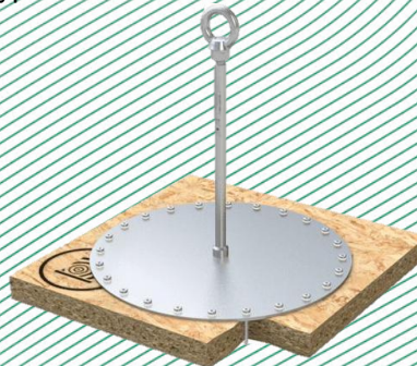
Fig. 14: Anchor device, type: ABS-Lock® X-H-24
