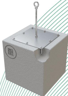
Fig. 13: Anchor device, type: ABS-Lock® X-Y
