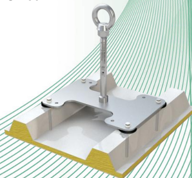
Fig. 12: Anchor device, type: ABS-Lock® X-SW
