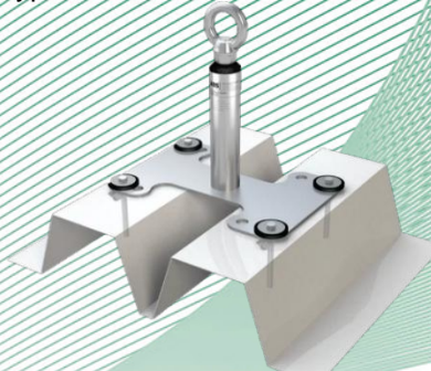
Fig. 16: Anchor device, type: ABS-Lock® X-T-21
