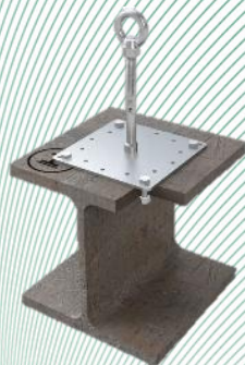
Fig. 7: Anchor device, type: ABS-Lock® X-ST
