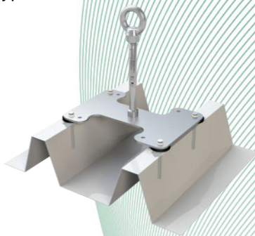
Fig. 15: Anchor device, type: ABS-Lock® X-T
